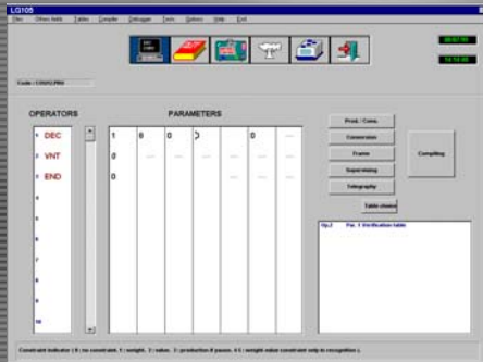
Decoder definition
